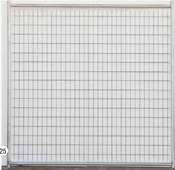
6-Ga Hot Dipped Galvanized 2x4 Welded Wire Panels
